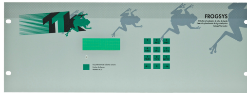
FG-SYS E, Digital Unit Rack Mounted in 4U and 19" . Width: 484 mm and High: 176 mm
